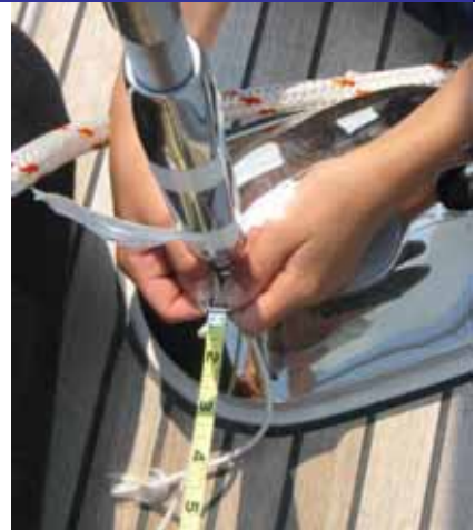
Measuring aft from the shroud base. Note the taped cotter pins to prevent snagging of sheets or shins.
