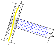
1 to 3 rows of contrasting 3-step stitching and internal leechline chafe guard
